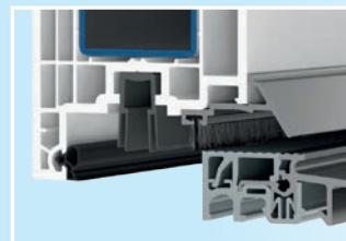
Detail prahu
